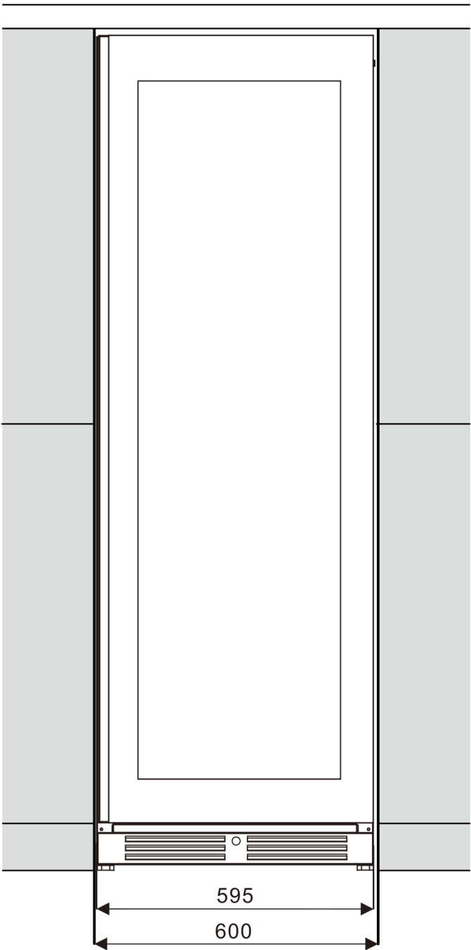
Front View
