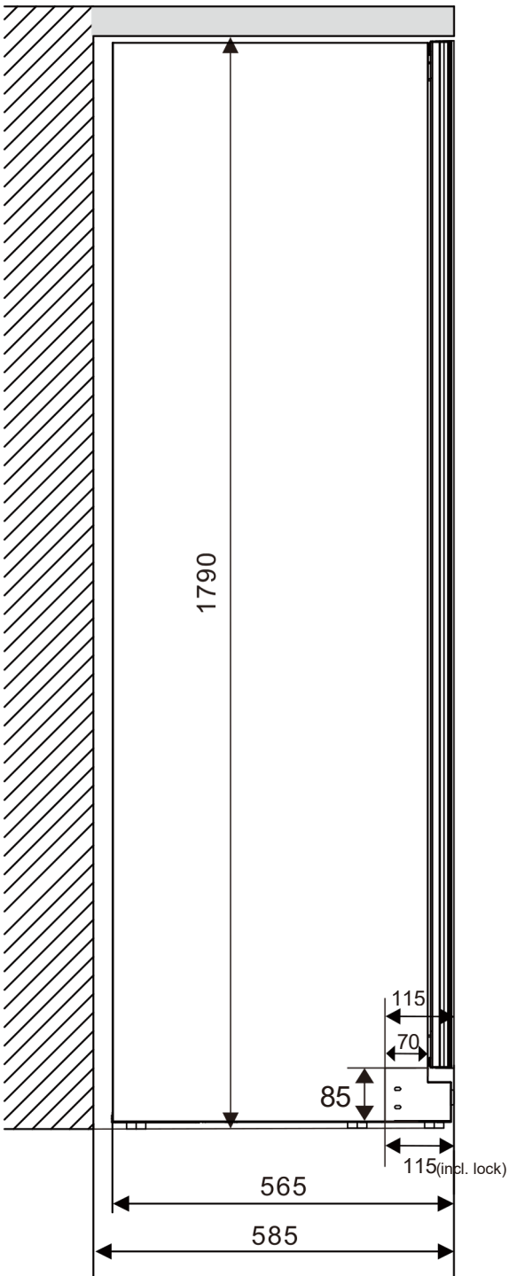
Side View
